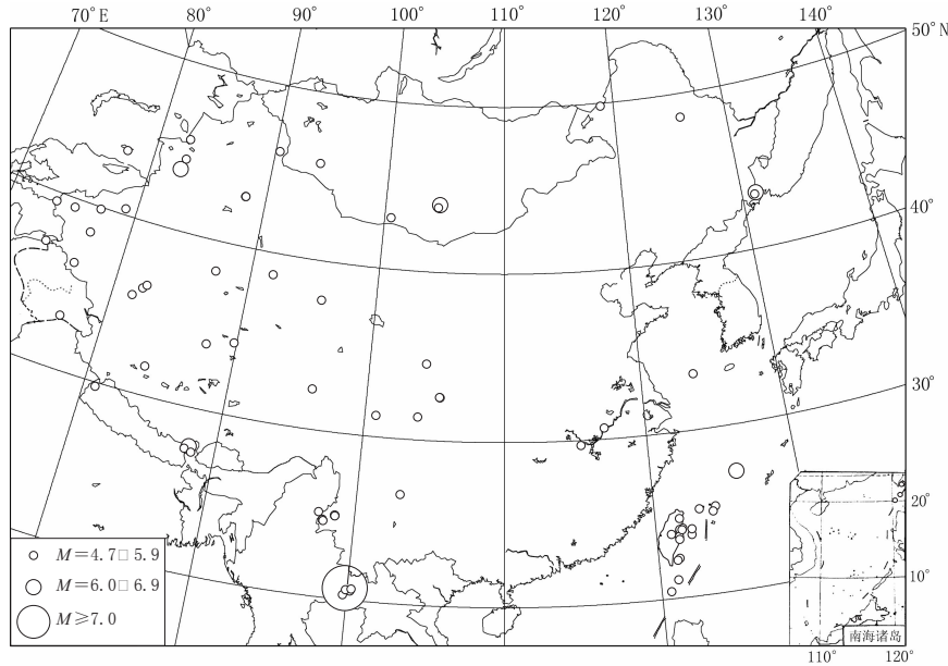
2011 年中国及邻区地震震中分布图 Epicentral distribution in and near China in 2011
