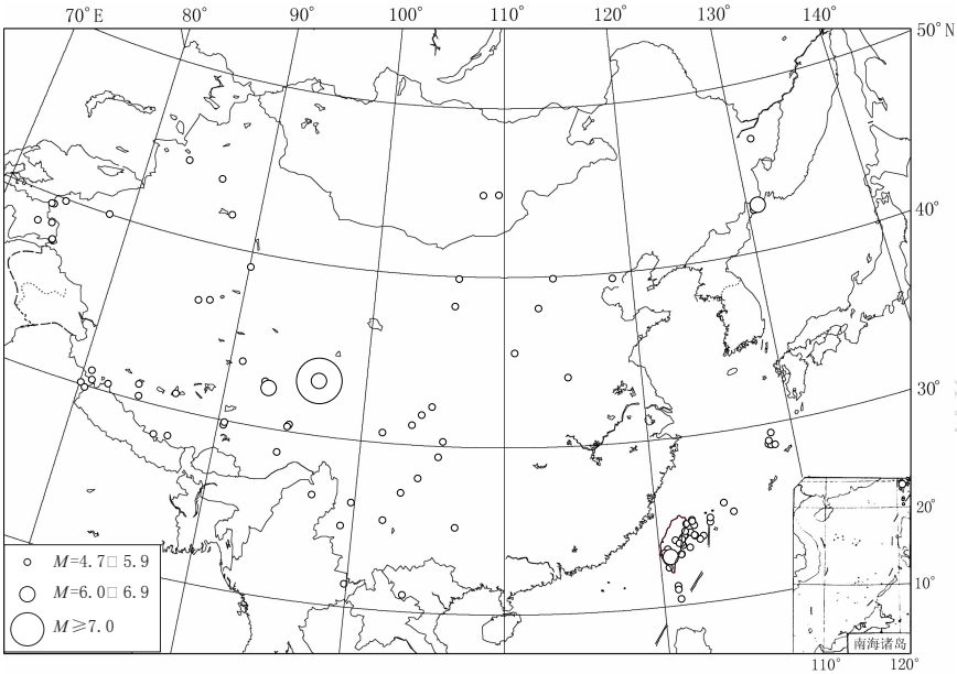
2010 年中国及邻区地震震中分布图 Epicentral distribution in and near China in 2010
