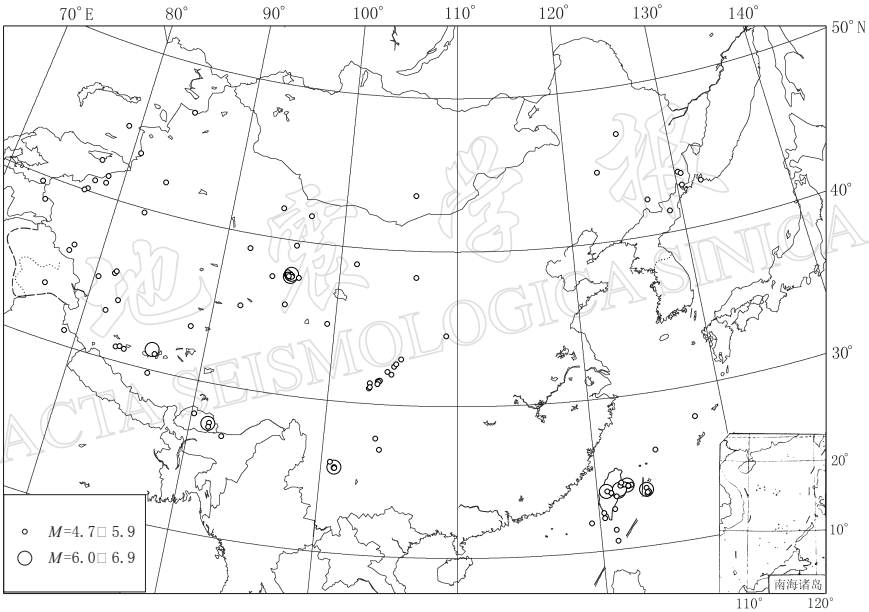
2009 年中国及邻区地震震中分布图 Epicentral distribution in and near China in 2009
